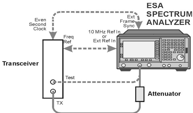
Figure 4-8 Alternative Measurement Setup
