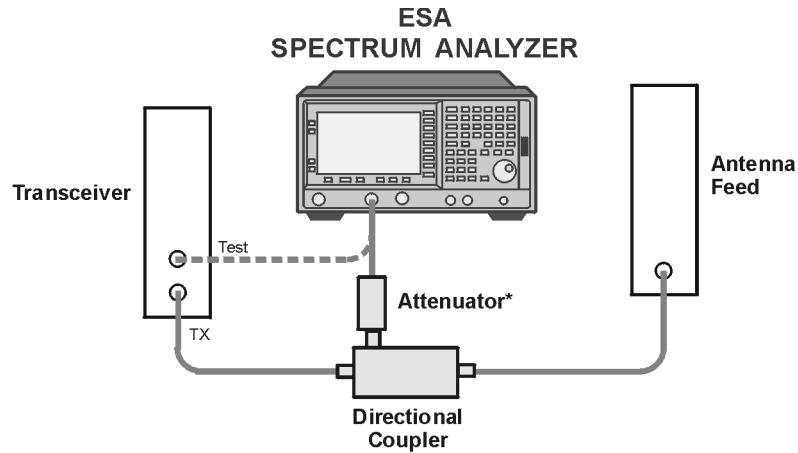
Figure 3-5 Measurement Setup
