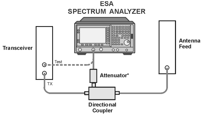
Figure 3-21 Measurement Setup
