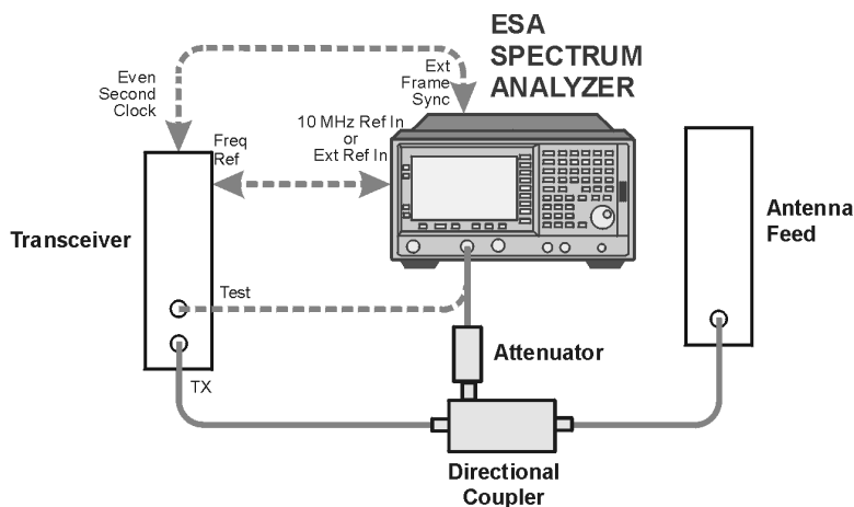
Figure 4-7 Measurement Setup
